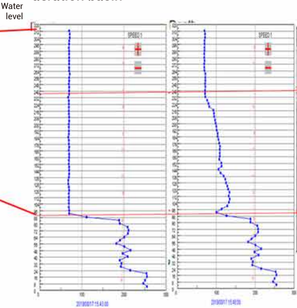
Activated sludge profiling in aeration basin
