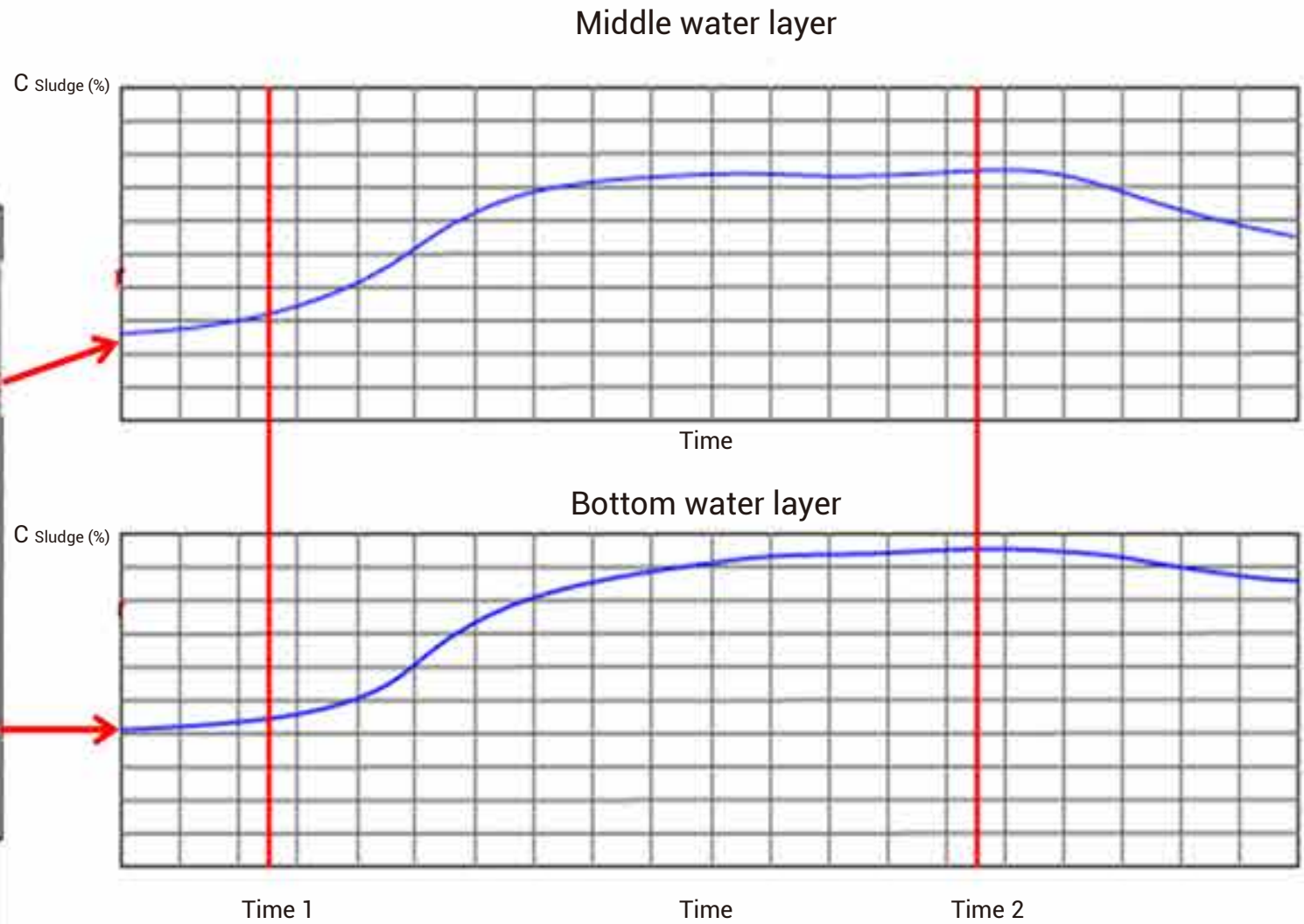
Time series profiling concentration vs time Time-concentration profiling (T-C profiling) at any specific location
