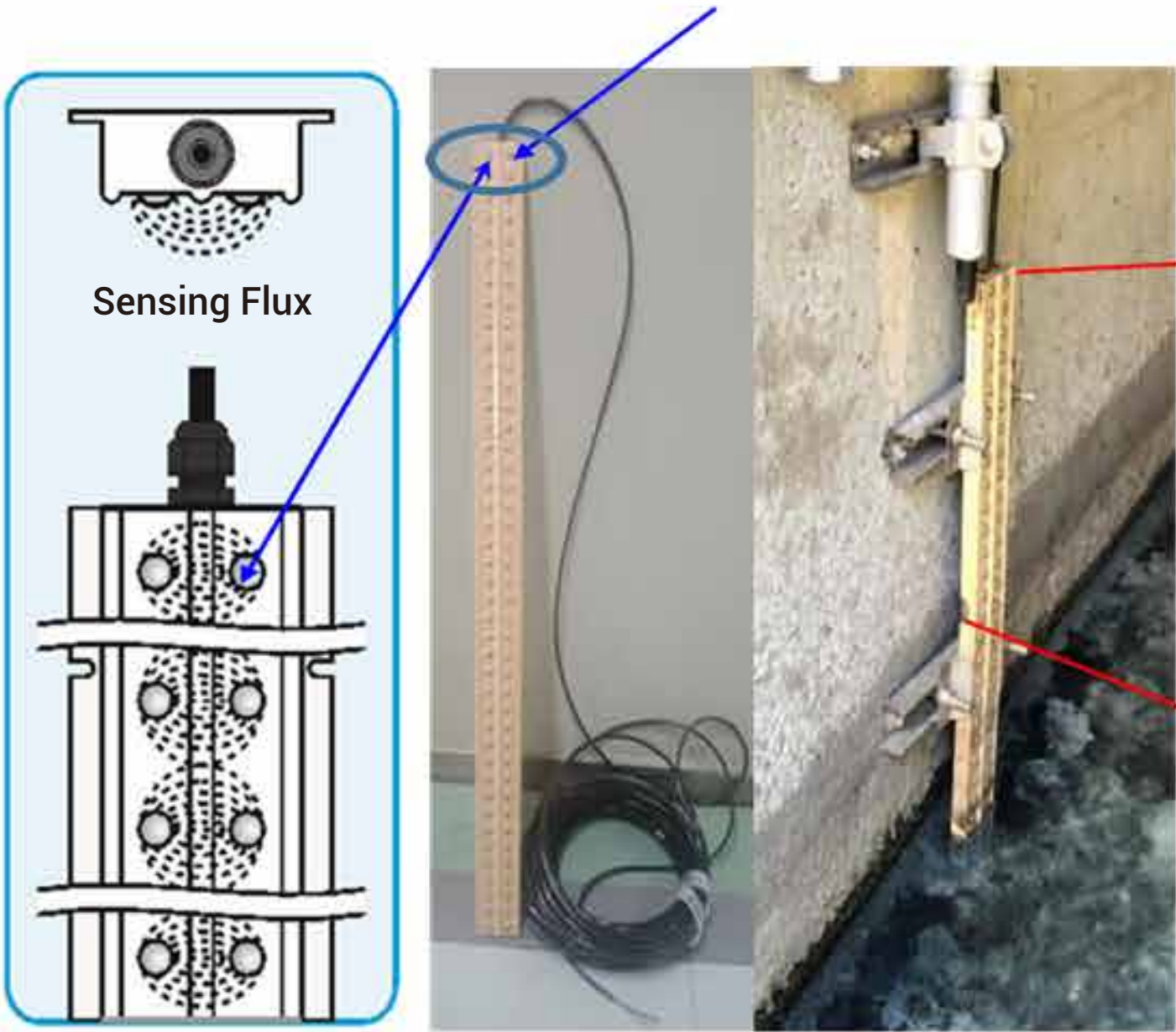
Activated sludge profiling in aeration basin
